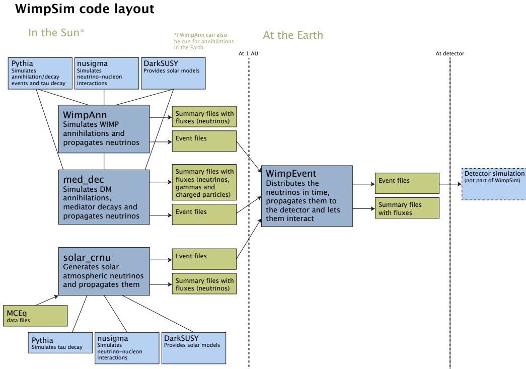
Figure 1: The layout of the WimpSim program with the four parts WimpAnn, solar_crnu, med_dec and WimpEvent. In the figure we show the structure for neutrinos coming from the Sun. WimpAnn can also be run for WIMP annihilations in the Earth, where the breakpoint between WimpAnn and WimpEvent instead is at the production fluxes at the centre of the Earth.
